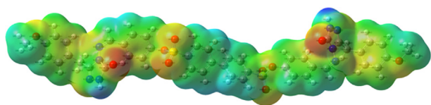
Fig. 3. MEP map of M7 inhibitor.
