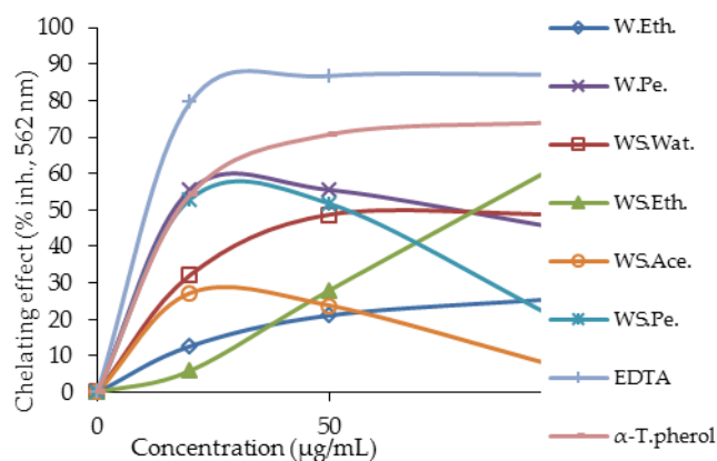
Figure 3. Metal chelating effect of different amount of the extracts, EDTA and \alpha -tocopherol on ferrous ions.
