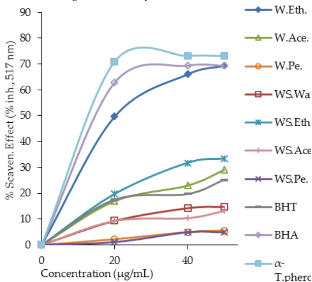
Figure 2. Scavenging effect of extracts, BHT, BHA and \alpha -tocopherol at different concentrations (20-40-50 \mu\text{g/mL} ).
