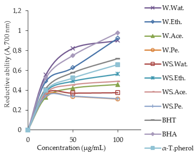
Figure 1. Total reductive potential of different concentrations of extracts, BHT, BHA and \alpha -
