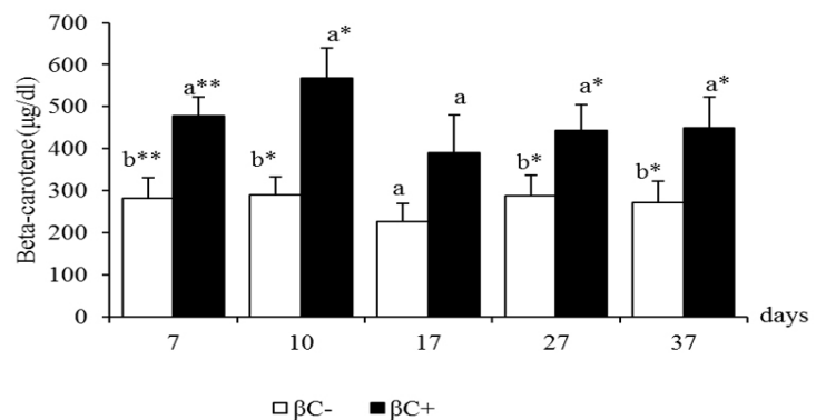
Fig 2. Comparison of mean beta-carotene concentrations ( \mu g/dL) during early pregnancy between groups
