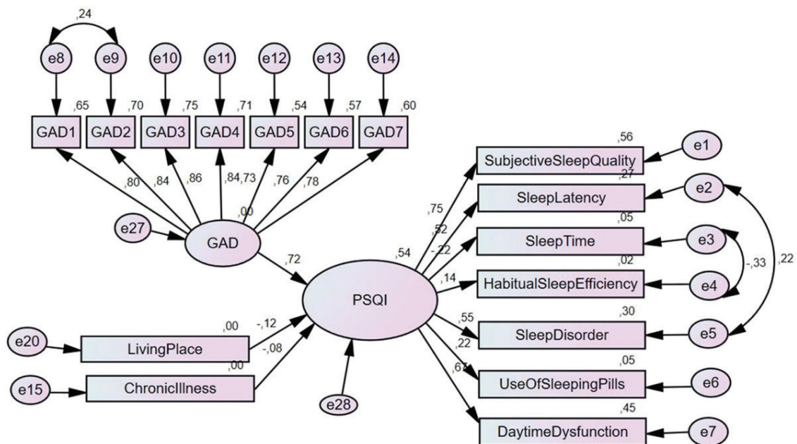
Figure 3. Revised model predicting the factors affecting sleep quality
