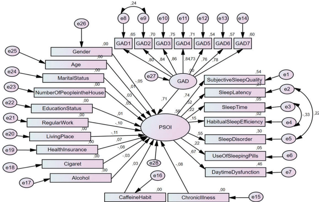
Figure 2. Initial structural equation model predicting factors affecting sleep quality
