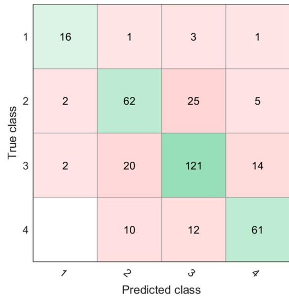
Fig. 3. Confusion matrix of decision tree in case 1.
